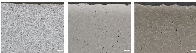
As sintered
